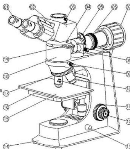
A5P.2603-BS Analyzer + Polarizer
