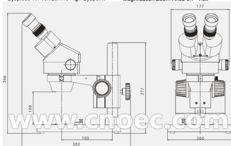
A23.0901 Zoom Stereo Microscope System Size
