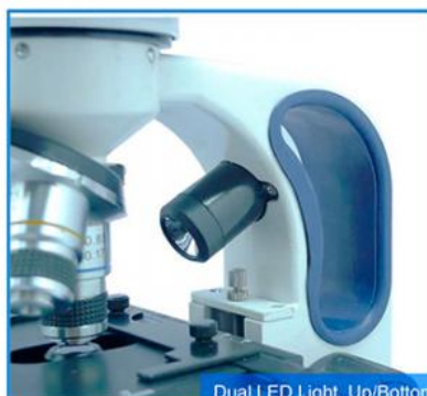
Dual LED Light, Up/Bottom Illumination, Brightness Adjustable
